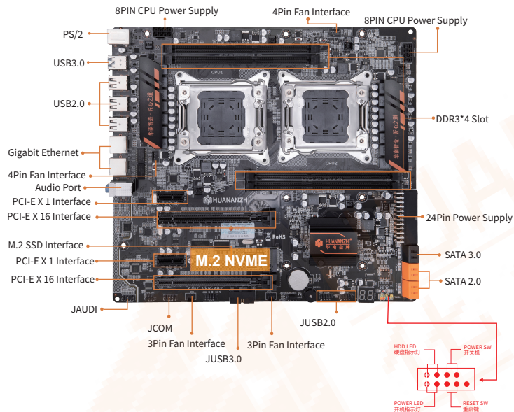
1-1 X79-4D DUAL LU Motherboard
