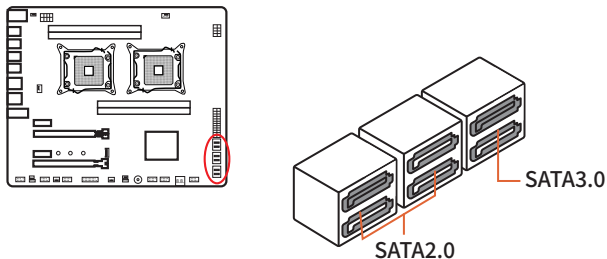
2-11 SATA Interface
